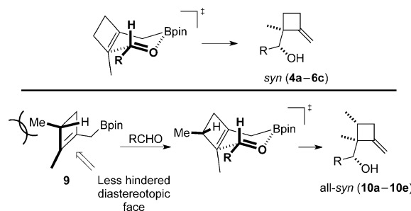
Scheme 4. Zimmerman–Traxler models explain the syn -diastereoselectivity in MCBs.
